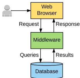
Figure 3: Architecture
